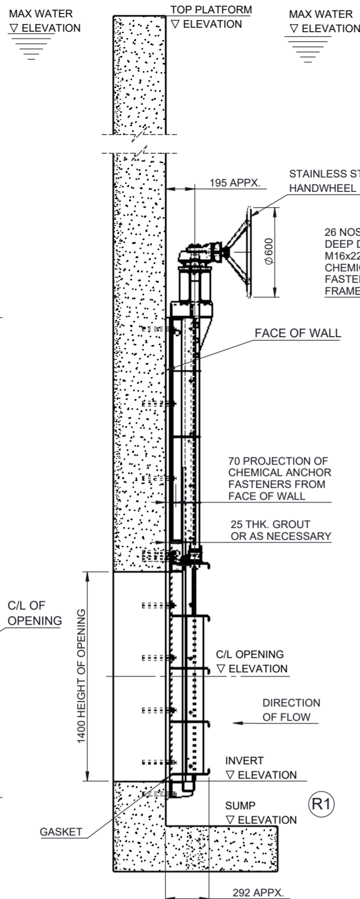
SIDE VIEW WITH CUT SECTION OF WALL
