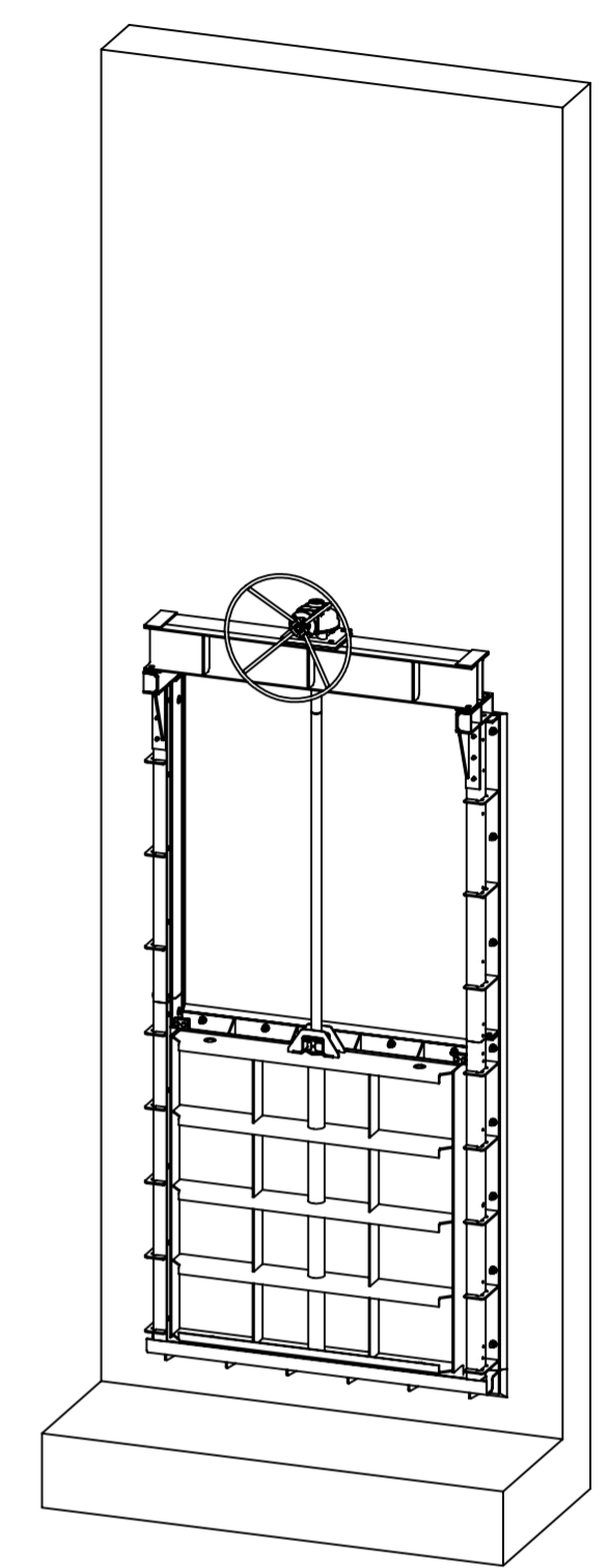
ISOMETRIC VIEW
