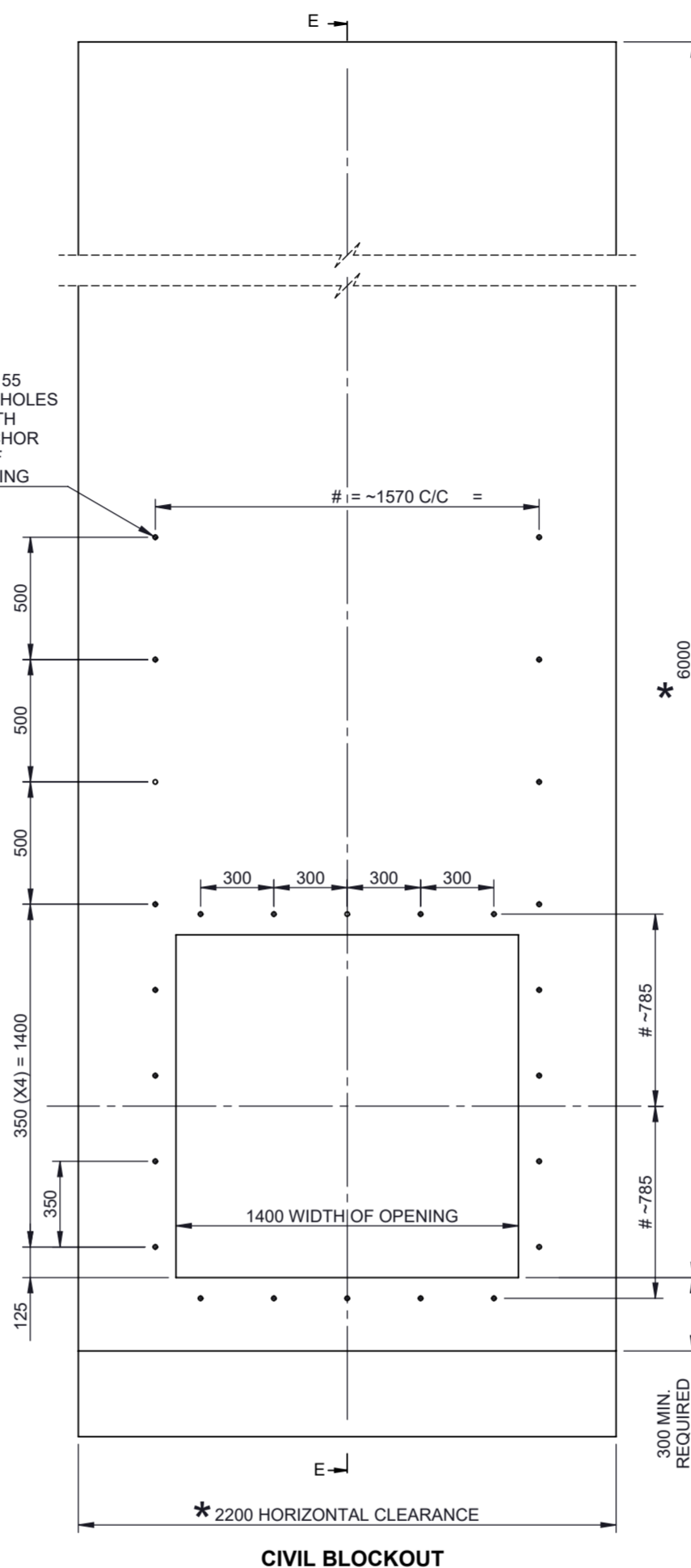
CIVIL BLOCKOUT
