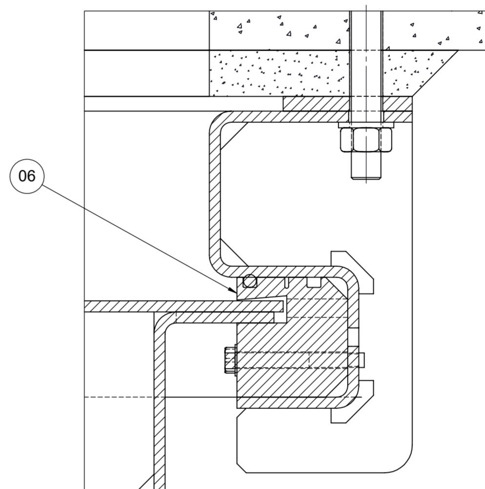
SIDE SEALING SECTION
