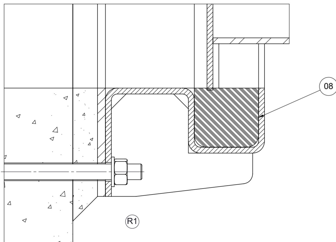
BOTTOM SEALING SECTION
