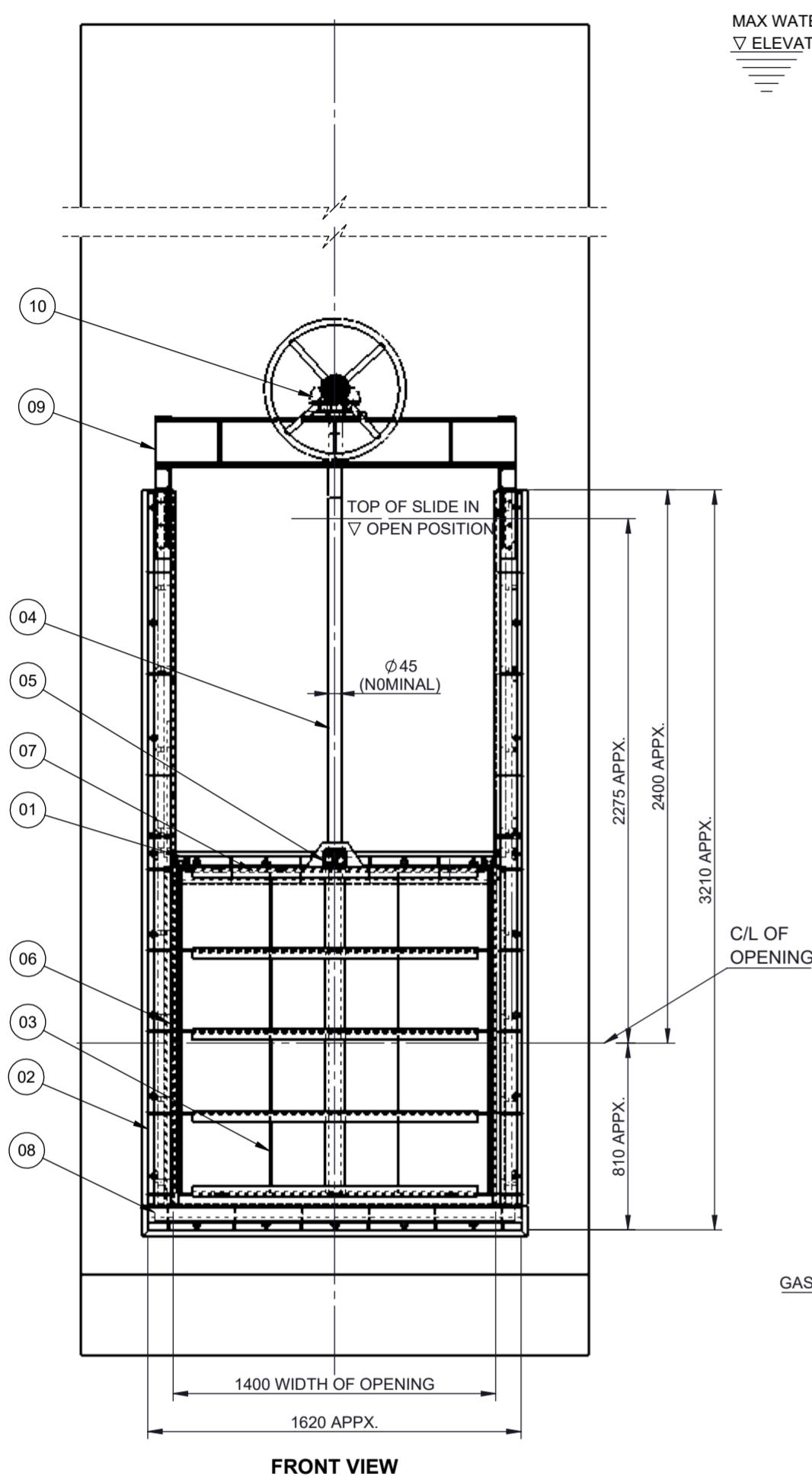
FRONT VIEW
