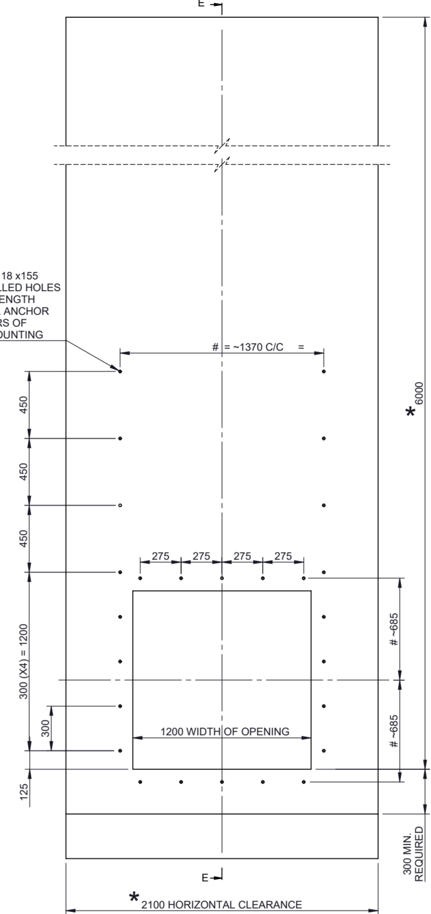
CIVIL BLOCKOUT
