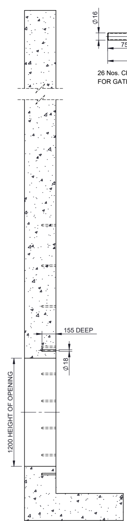
SECTION E-E
