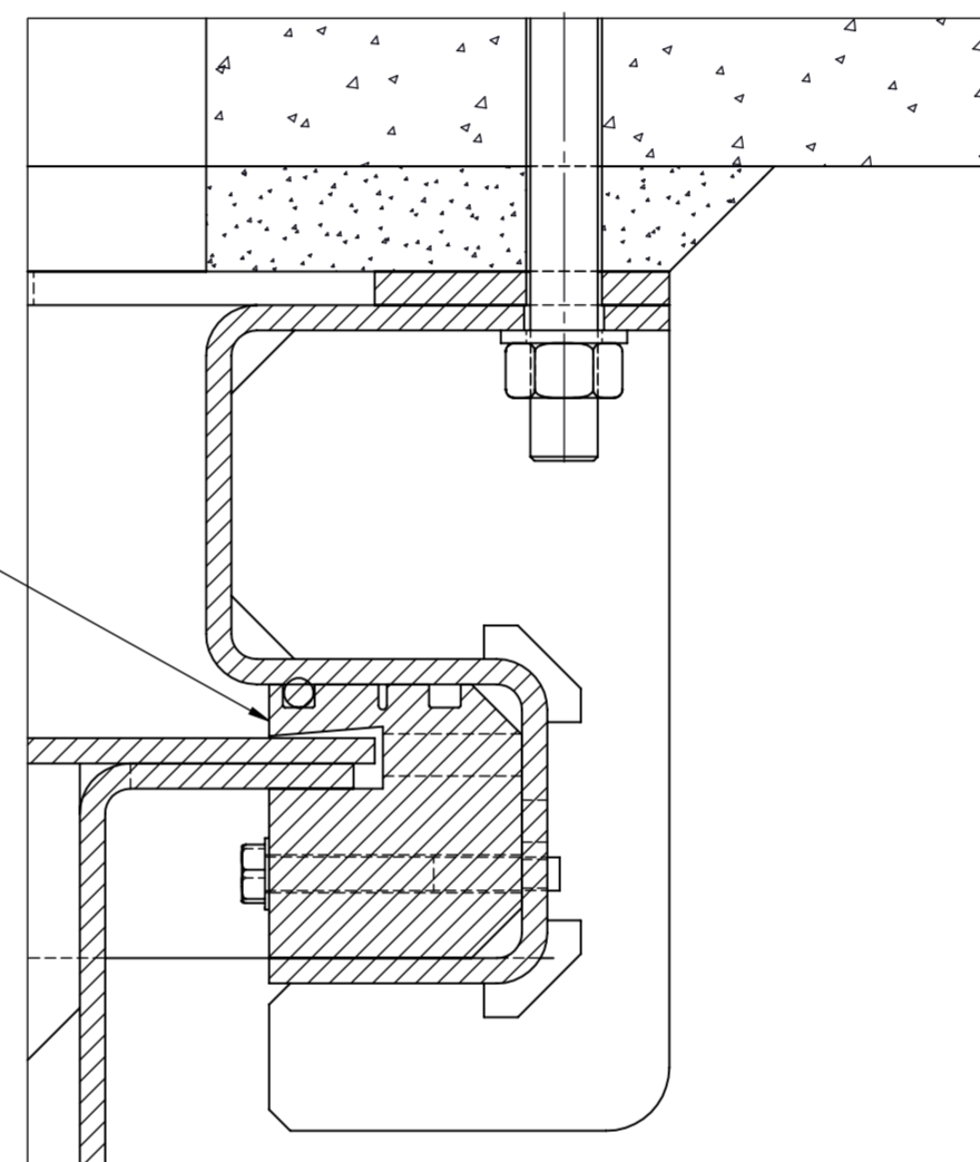
SIDE SEALING SECTION
