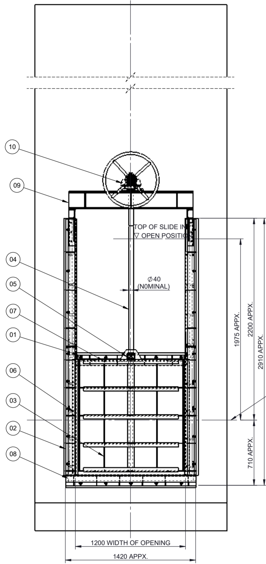
FRONT VIEW
