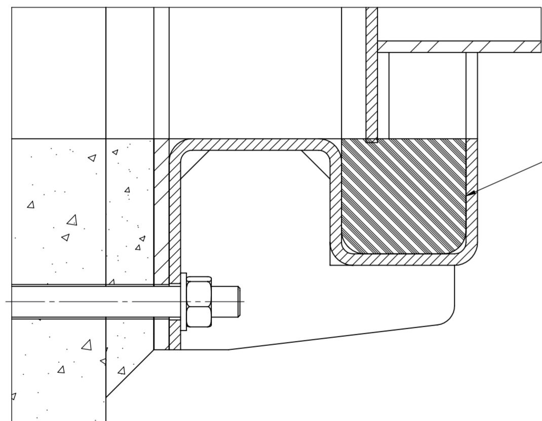
BOTTOM SEALING SECTION
