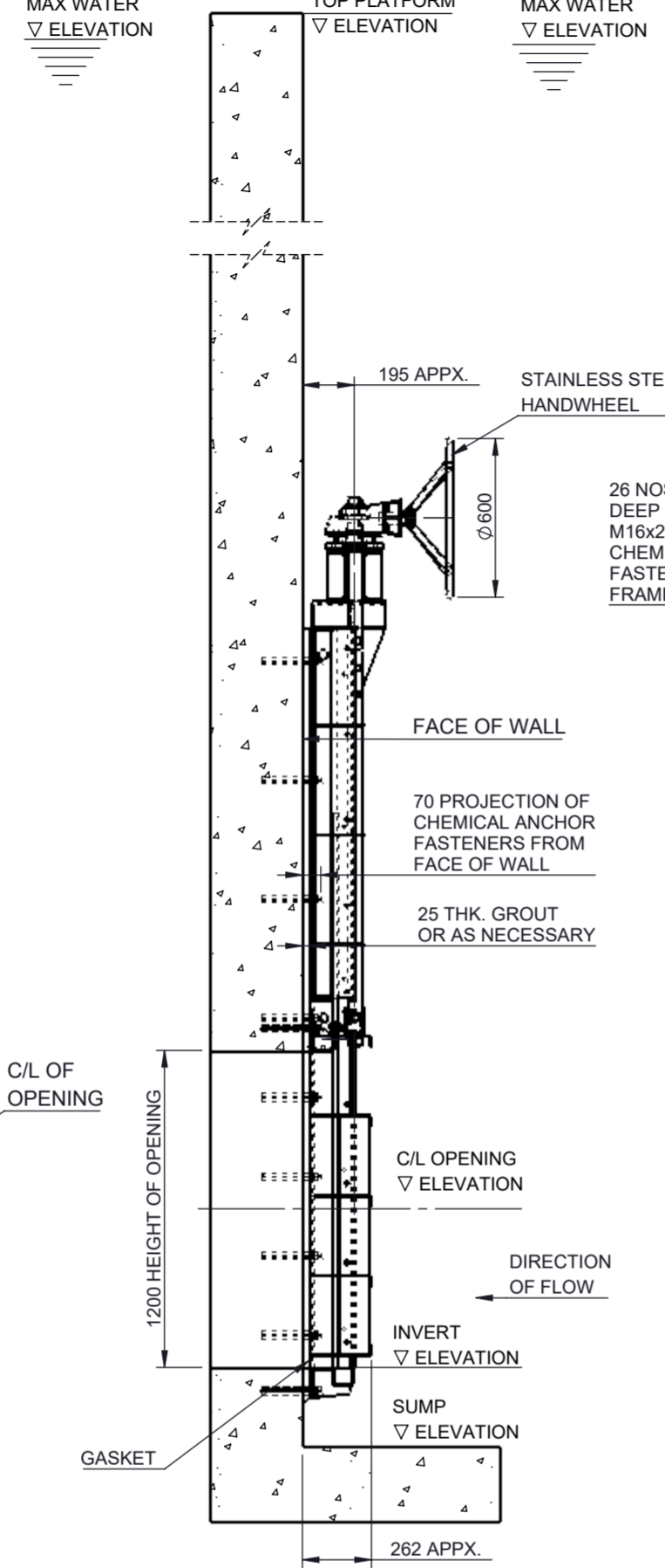
SIDE VIEW WITH CUT SECTION OF WALL
