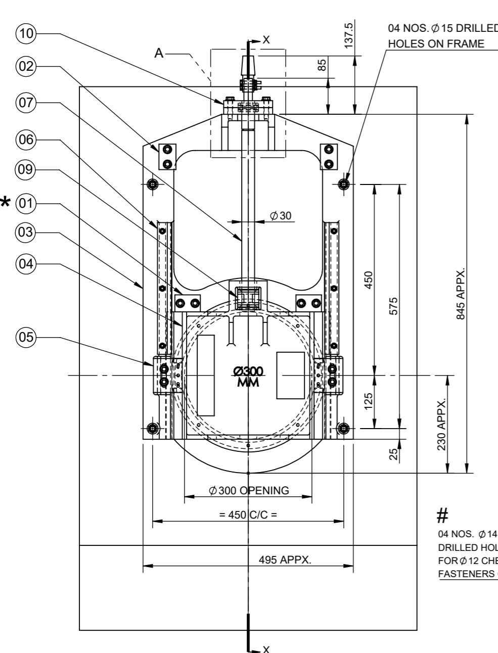
FRONT VIEW OF CAST IRON SLUICE GATE
