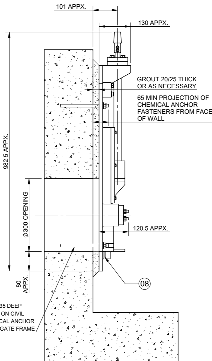
SIDE VIEW WITH CUT SECTION OF WALL
