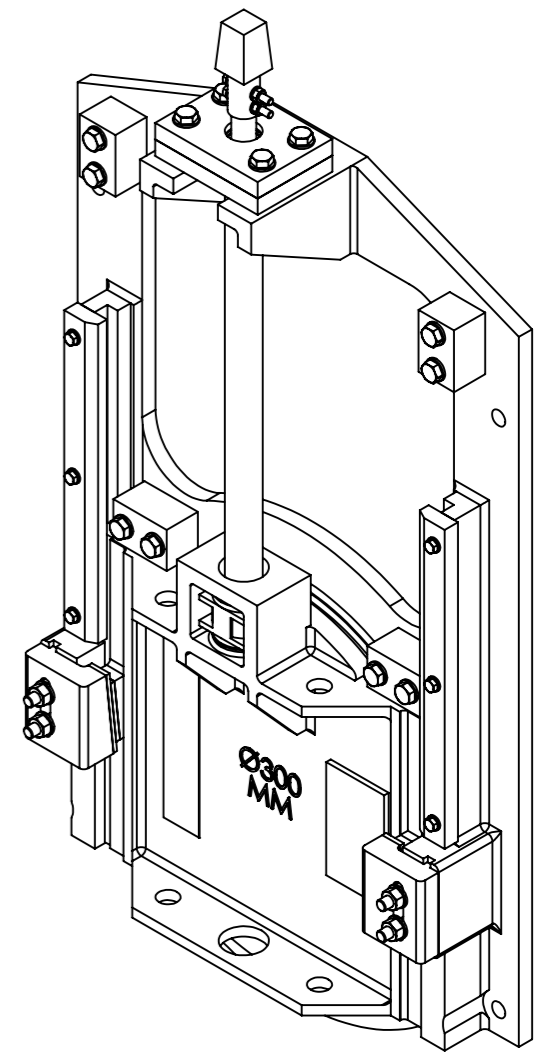
ISOMETRIC VIEW WITHOUT CIVIL
