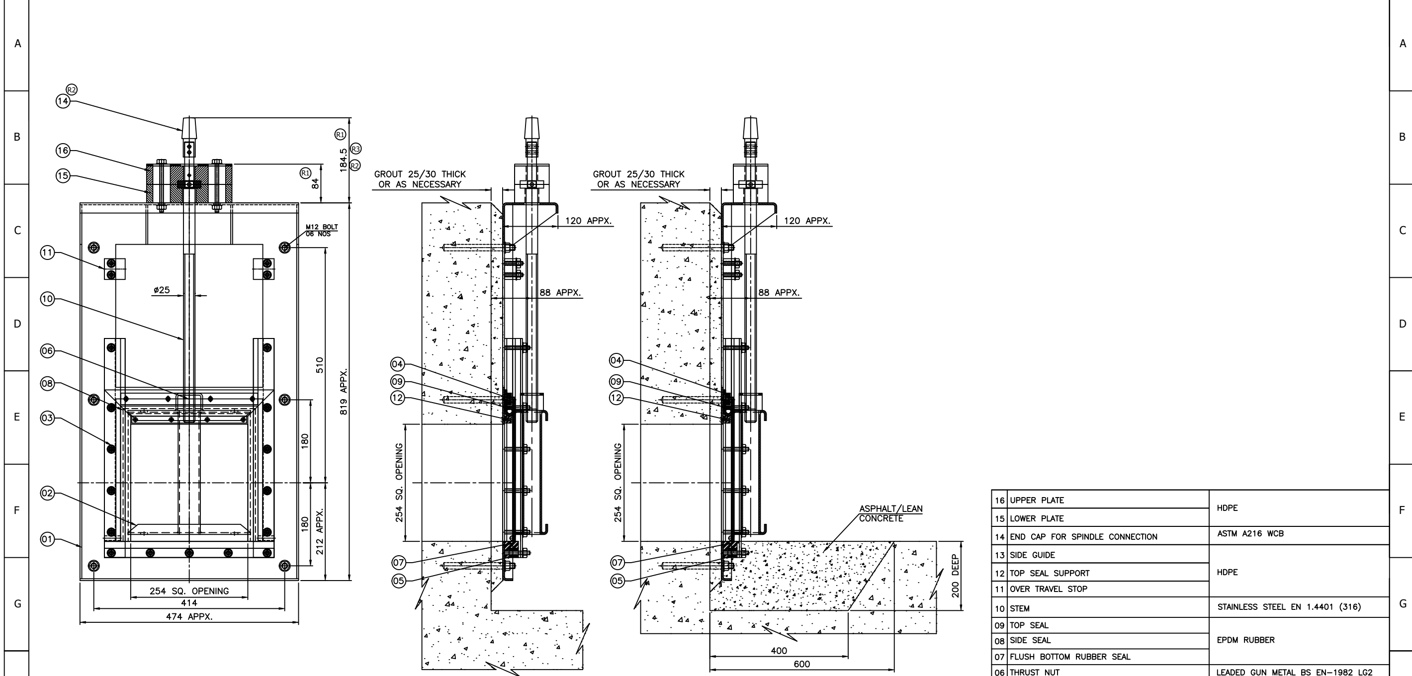
SIDE VIEW WITH CUT SECTION OF WALL FOR COVENTIONAL BOTTOM CLOSURE GATE
