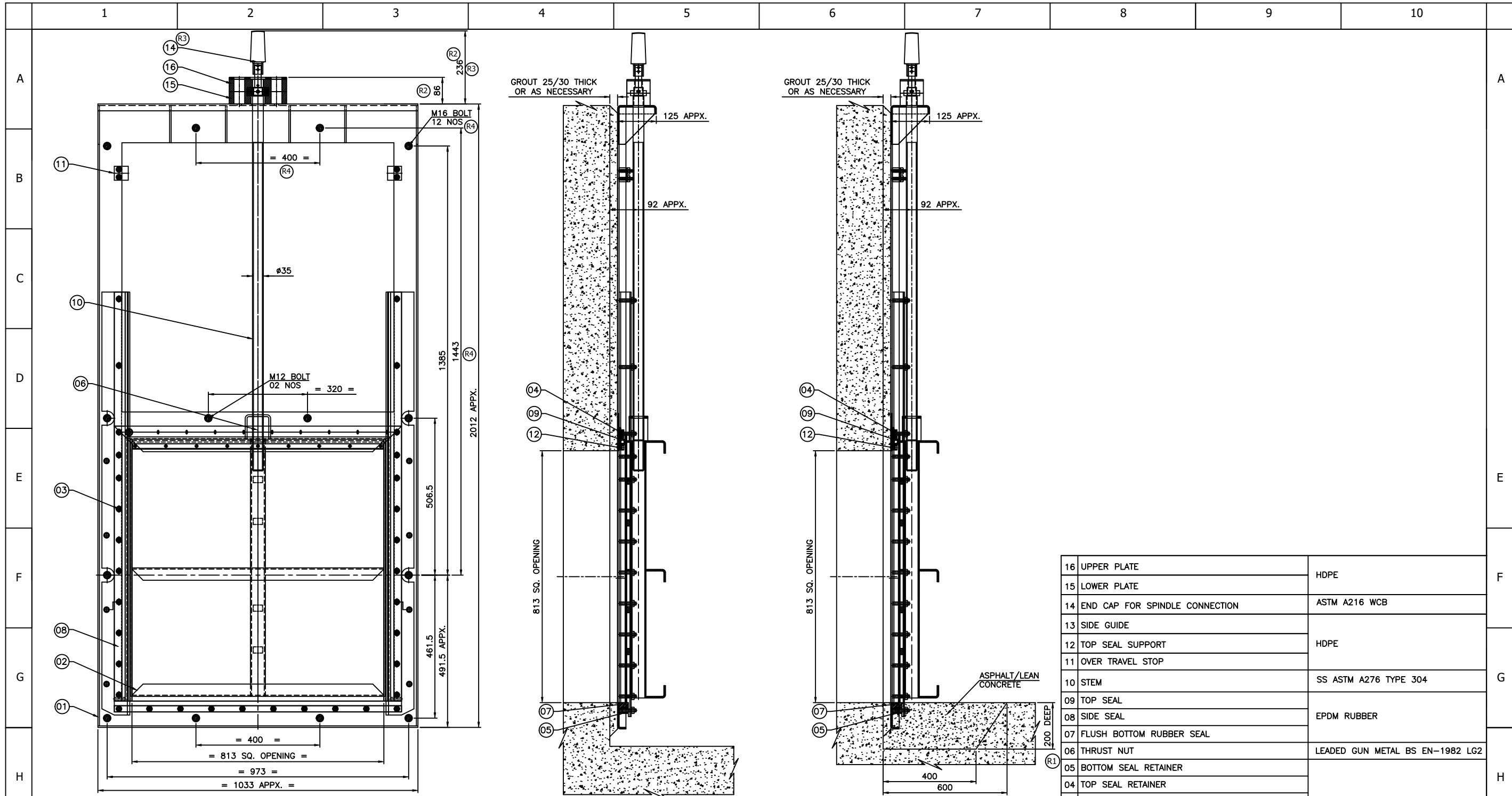
FRONT VIEW OF STAINLESS STEEL SLUICE GATE AFTER INSTALLATION SIDE VIEW WITH CUT SECTION OF WALL FOR COVENTIONAL BOTTOM CLOSURE GATE SIDE VIEW WITH CUT SECTION OF WALL FOR FLUSH BOTTOM CLOSURE GATE
