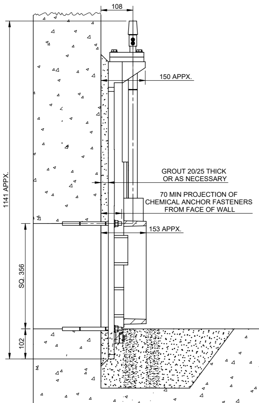
SIDE VIEW WITH CUT SECTION OF WALL
