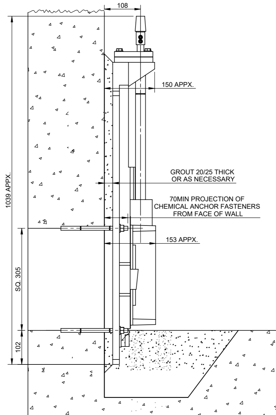
SIDE VIEW WITH CUT SECTION OF WALL
