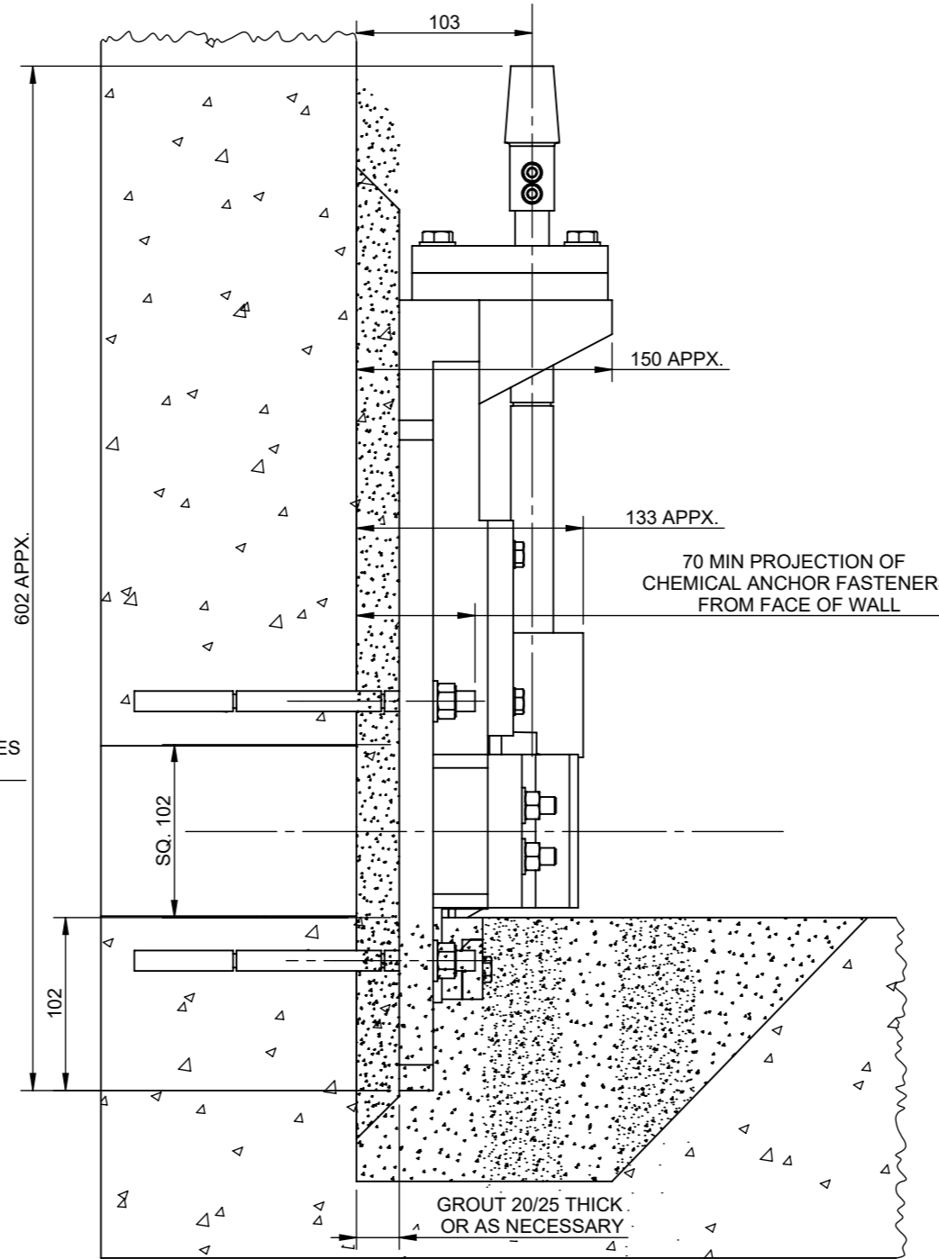
SIDE VIEW WITH CUT SECTION OF WALL
