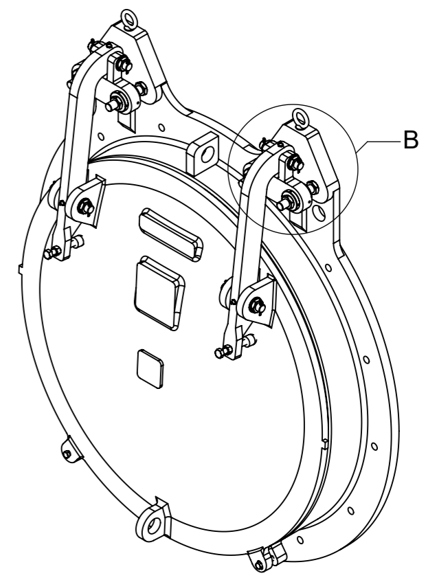
ISOMETRIC VIEW
