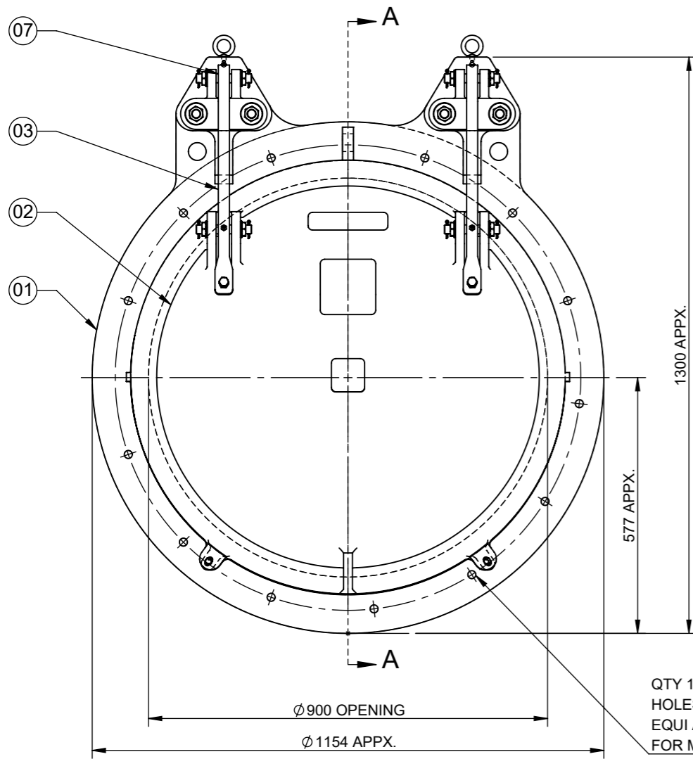
FRONT VIEW
