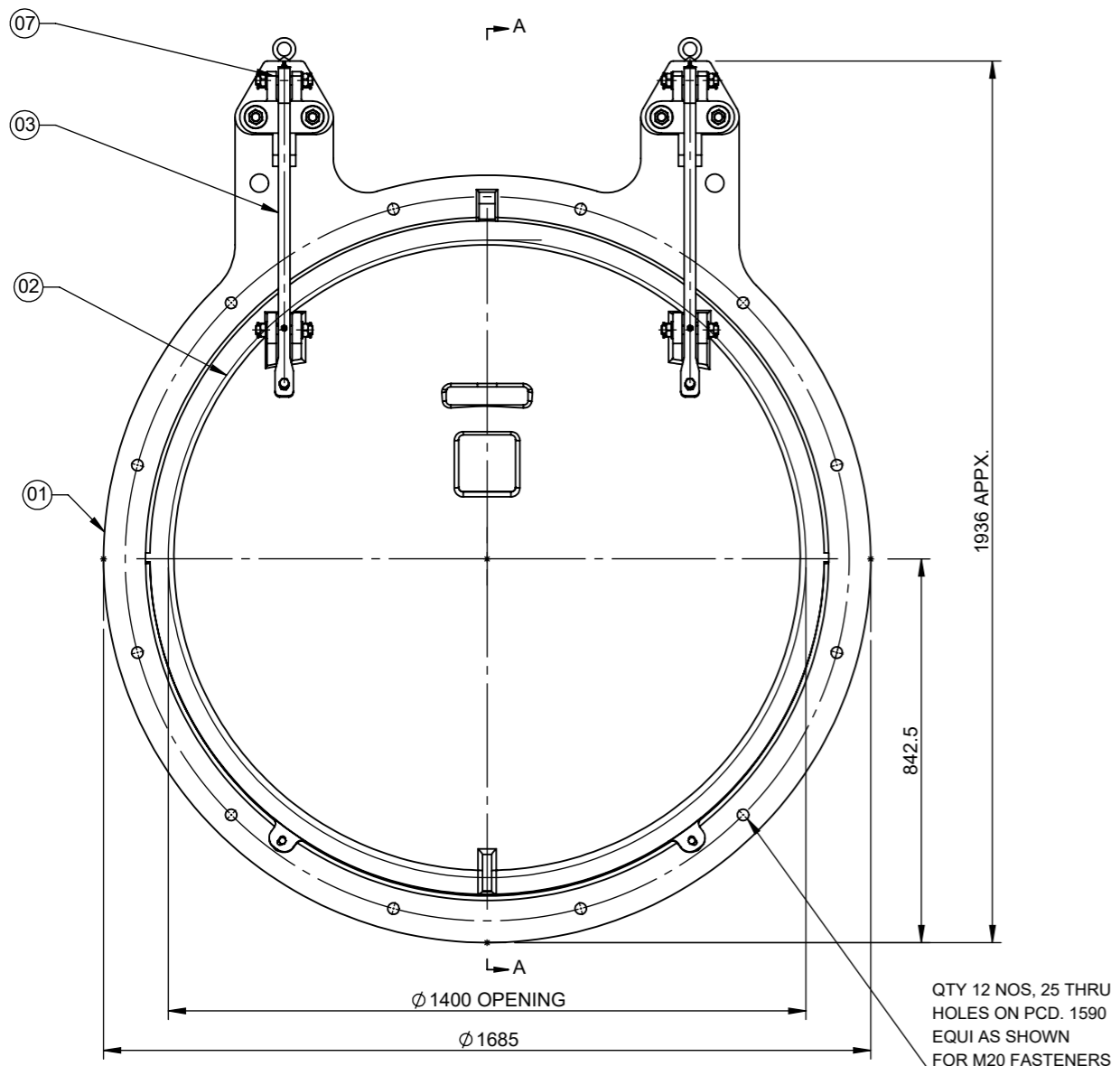
FRONT VIEW
