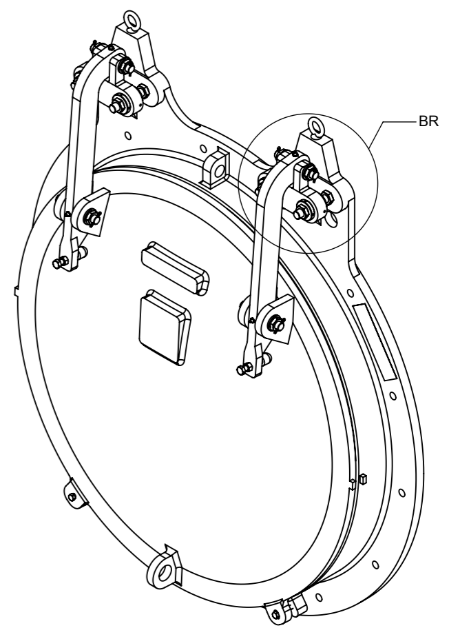
ISOMETRIC VIEW
