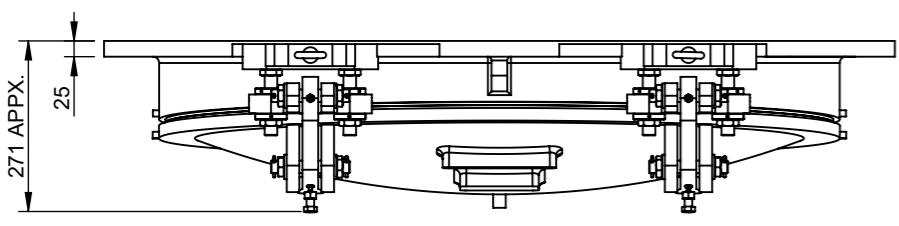
TOP VIEW
