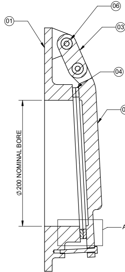
SECTION X-X
