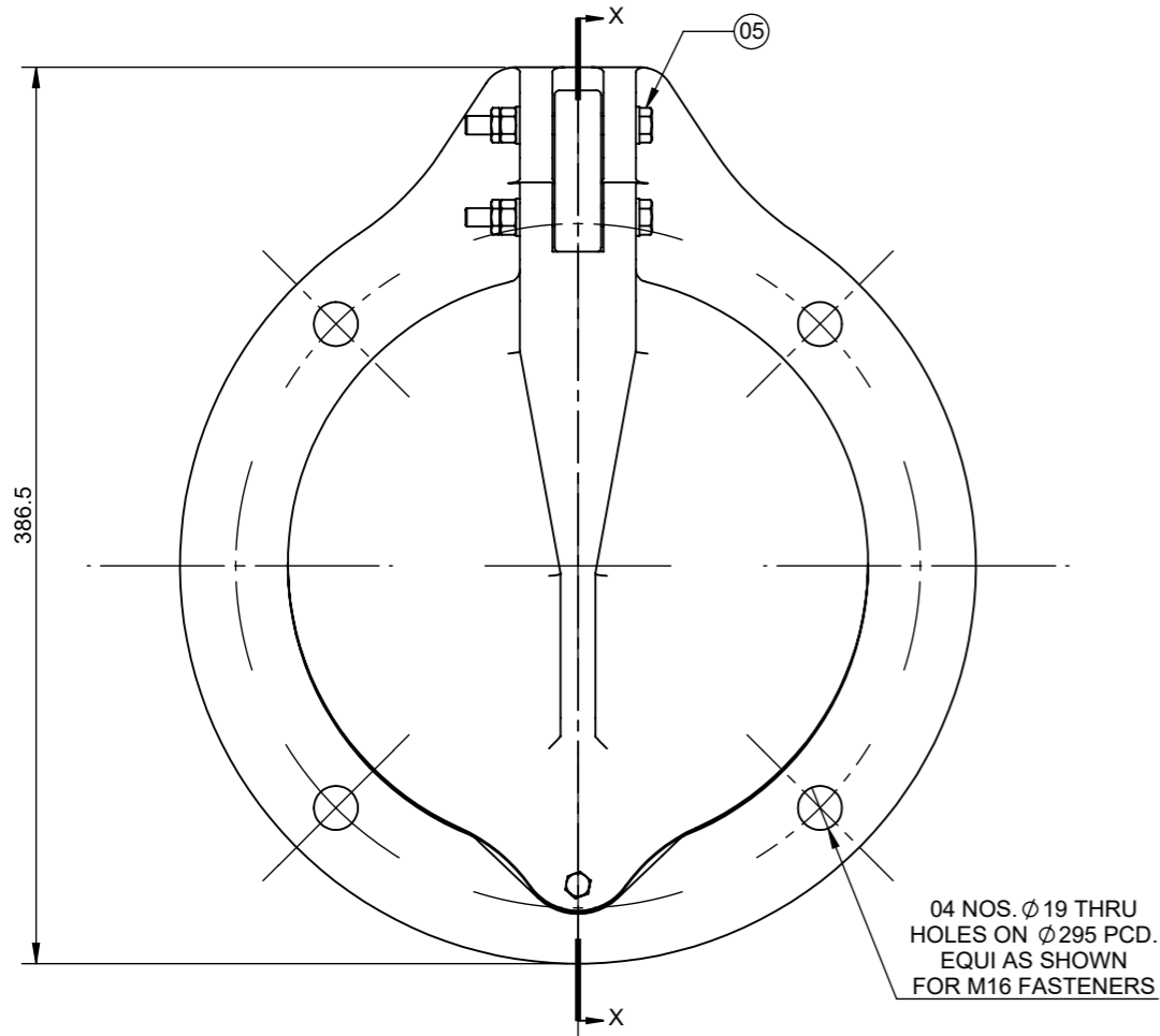
FRONT VIEW
