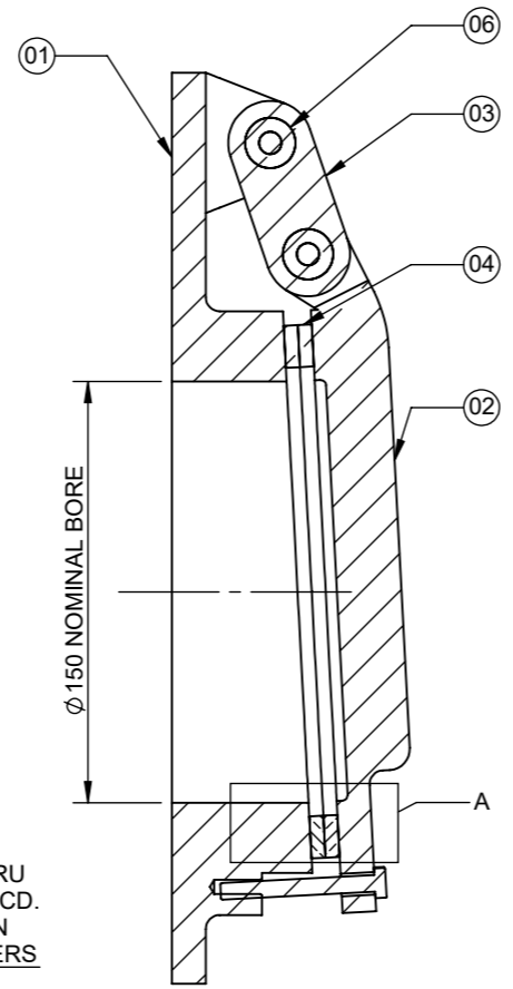
SECTION X-X
