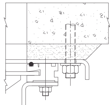
SIDE SEALING ARRANGEMENT
